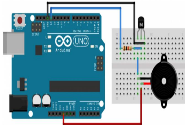
Gambar 4 Rangkaian Buzzer Arduino
