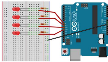
Gambar 3 Pemrograman 4 LED
