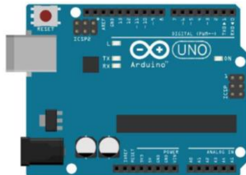
Gambar 2 Board Arduino Uno
