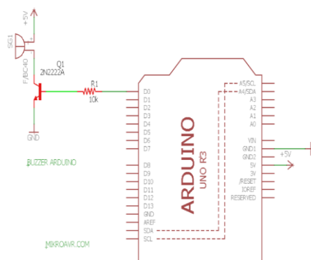
Gambar 5 Buzzer arduino
